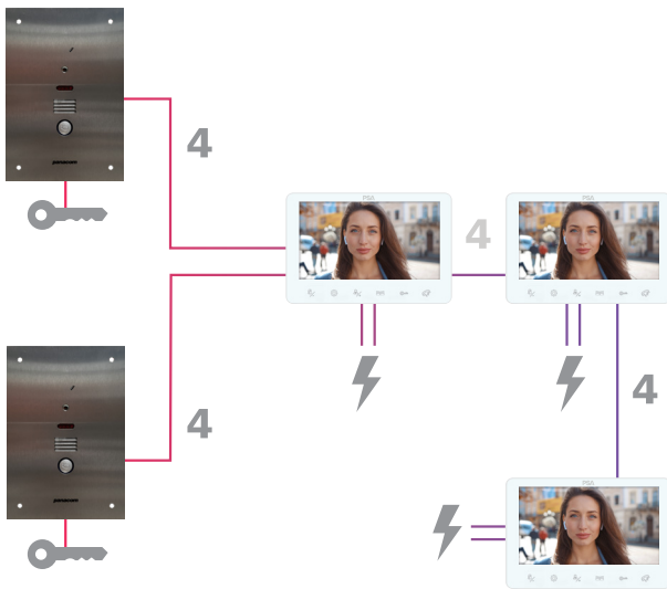
Max. System: 2 doors stations to 4 internal monitors
