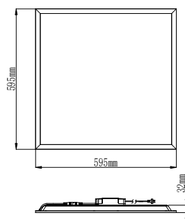
36W 595x595x32mm
