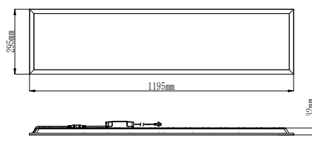
36W 1195x295x32mm
