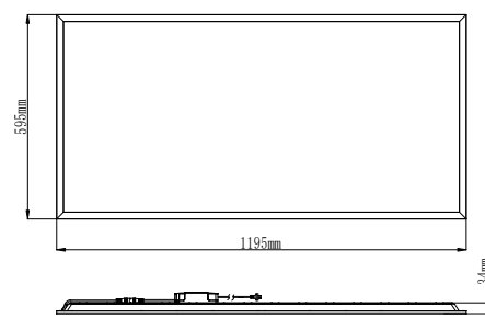
65W 1195x595x34mm
