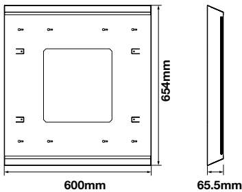
LDVPANSMF0606 600x654x65.5mm
