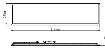
33/27W 1195x295x32mm
