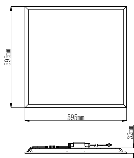
33/27W 595x595x32mm
