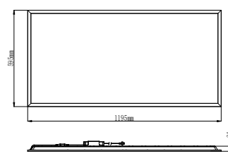
49/45W 1195x595x34mm
