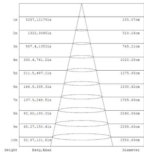
Diagram for RSNXCCT3DA-04 in 200W 4000K. Other diagrams available on request
