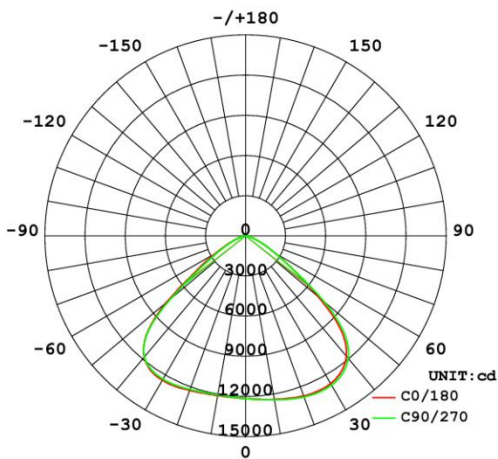
Diagram for RSNXCCT3DA-04 in 200W 4000K. Other diagrams available on request
