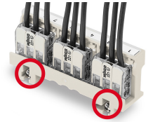
Mounting type (275 V) Mounting the carrier using conductive screws.
