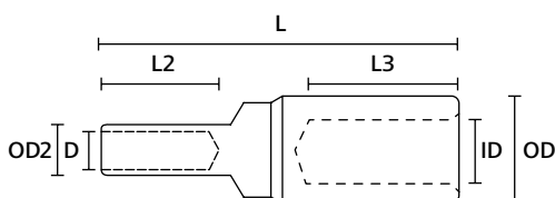
Bi-Metal Reducing Link, Side View
