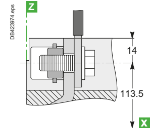
Bars/cables with lugs
