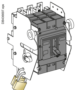
Chassis locking in the connected position
