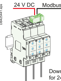
Supply, with the Communication function, via the Modbus interface
