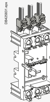
With 240 mm 2 cable connector for NSX100 to 250
