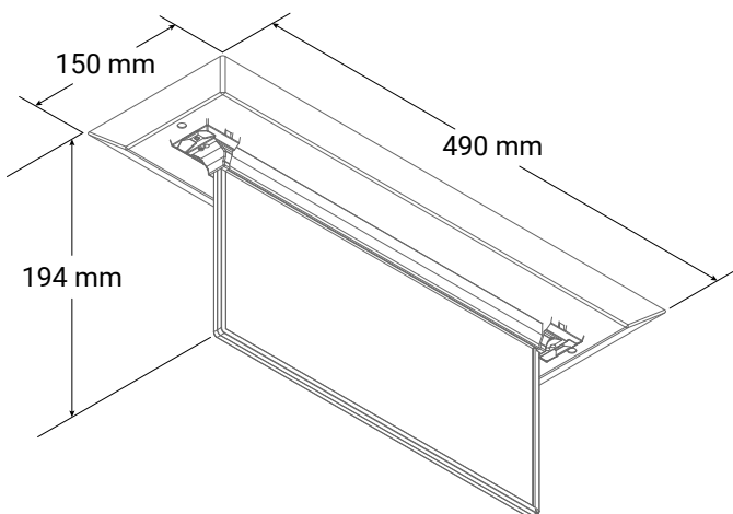
ORTHOGRAPHIC DRAWING
