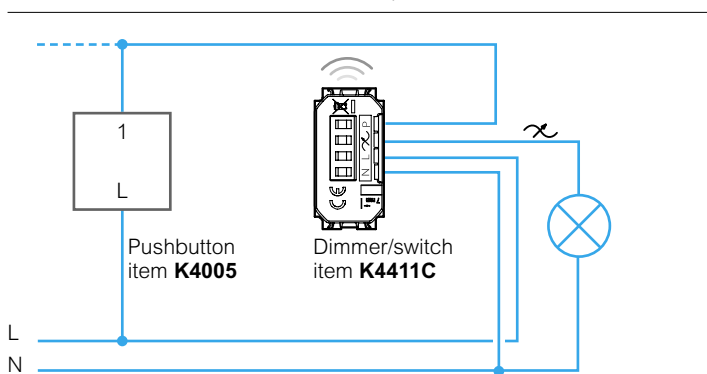
Dimmer/switch item K4411C with remote pushbuttons
