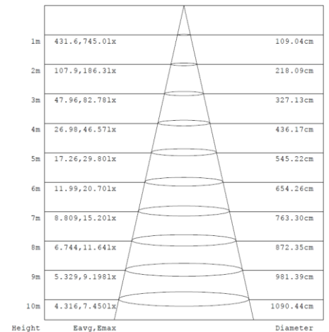
Diagram for RCS8CCT4-01 in 3000K. Other diagrams available on request
