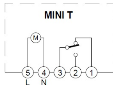
CIRCUIT CONNECTION
