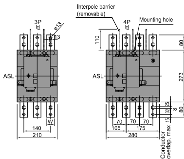
Rear Connected With Motor Operator
