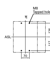
Drilling plan (front view)
