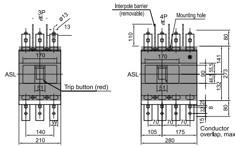
Front Connected With Extension Bars (Optional)
