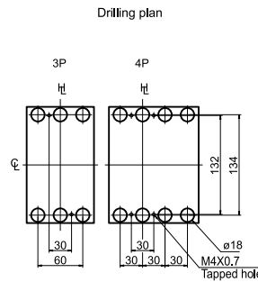
Drilling plan
