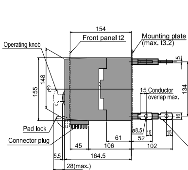
Rear Connected With Motor Operator
