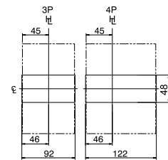
Panel cutout (Front view)
