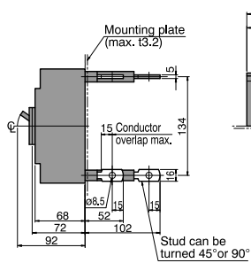
Front Connected With Motor Operator
