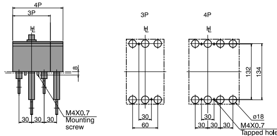
Drilling plan
