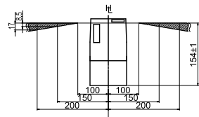
Panel hinge position (hatching area) bottom view
