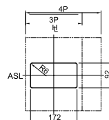
Panel cutout (front view)
