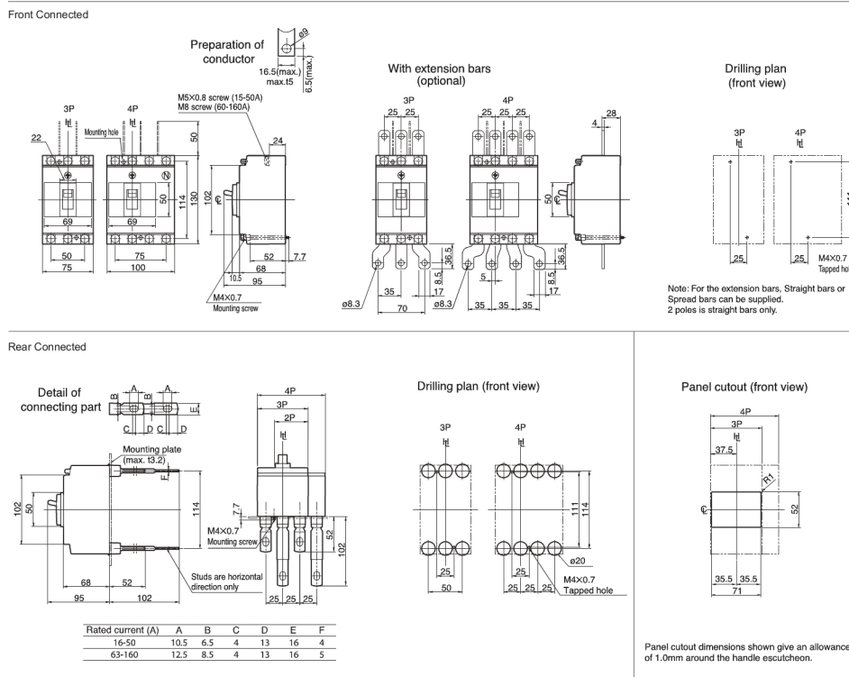
Dimension Diagram
