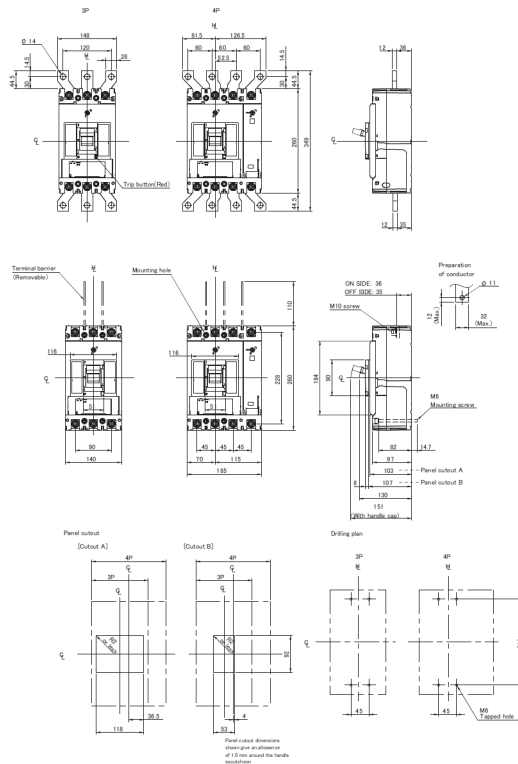
Dimension Diagram
