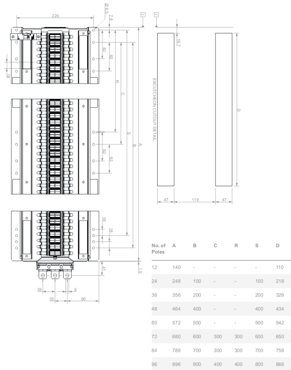
Dimension Diagram
