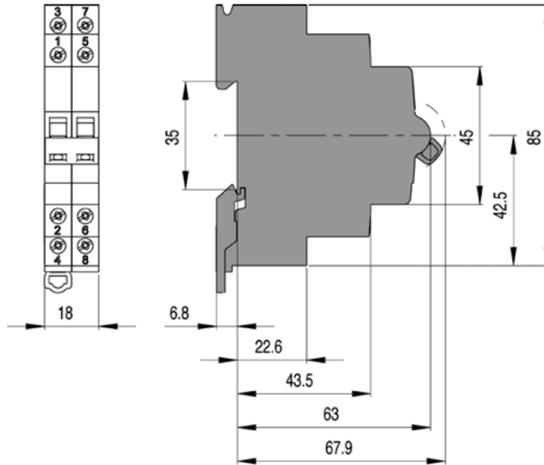
Dimension Diagram
