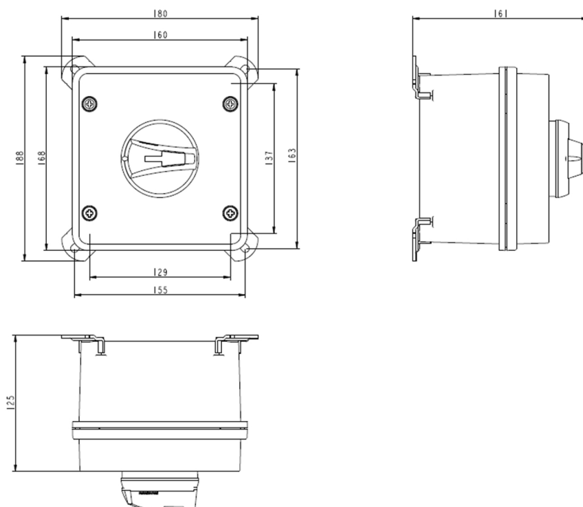
Dimension Diagram
