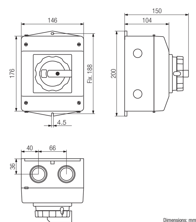
Dimension Diagram
