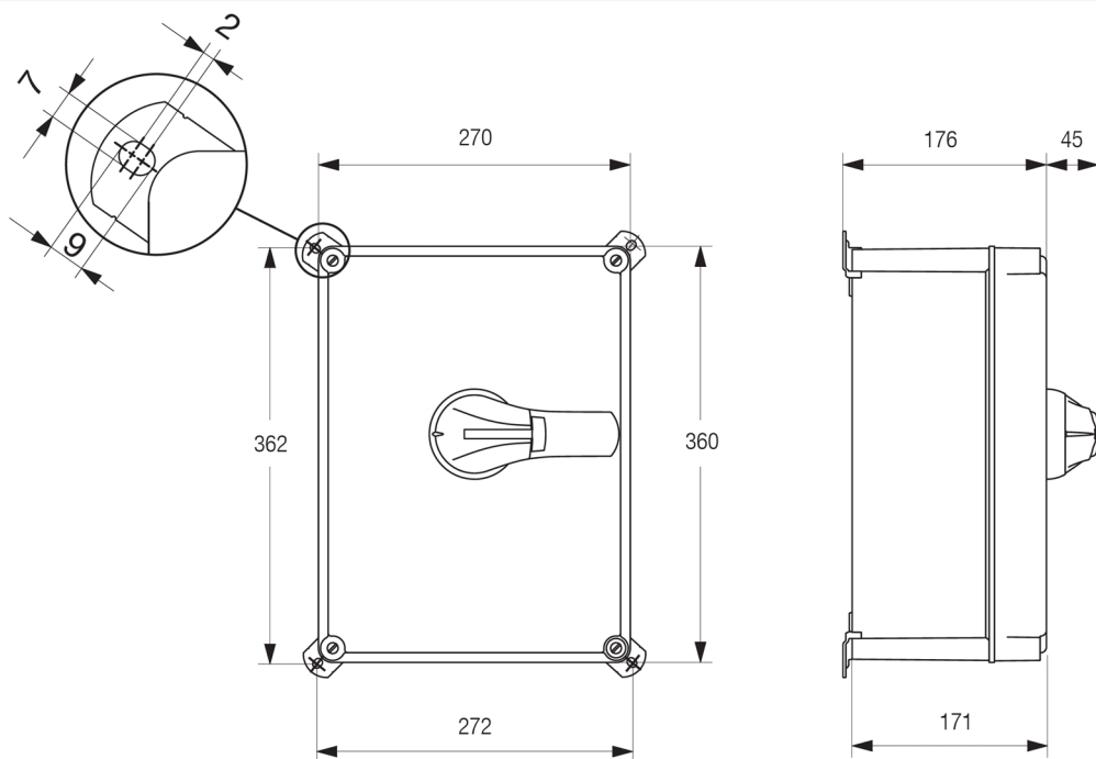
Dimension Diagram
