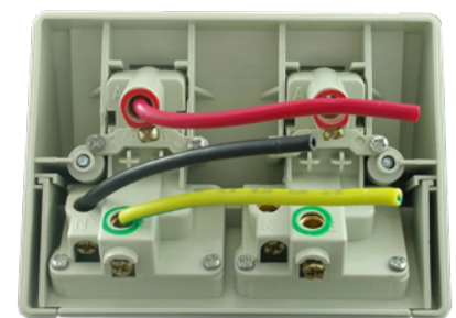
Separate Switch Wiring
