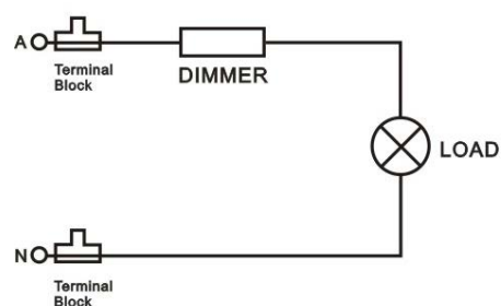
Electronic Dimmer (MTDM350)
