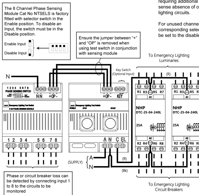
Connection / Wiring Diagram
