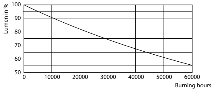
Lumen Maintenance Diagram - DN029B G2 LED12/CCT PSR-E D150 CAU
