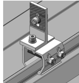
Install with Tin Interface
