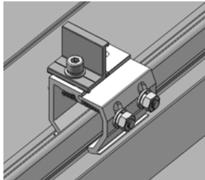
Install with Cross Connector Clamp of ECO-Rail
