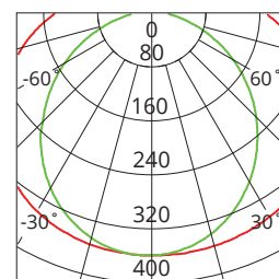
Photometric Diagram
