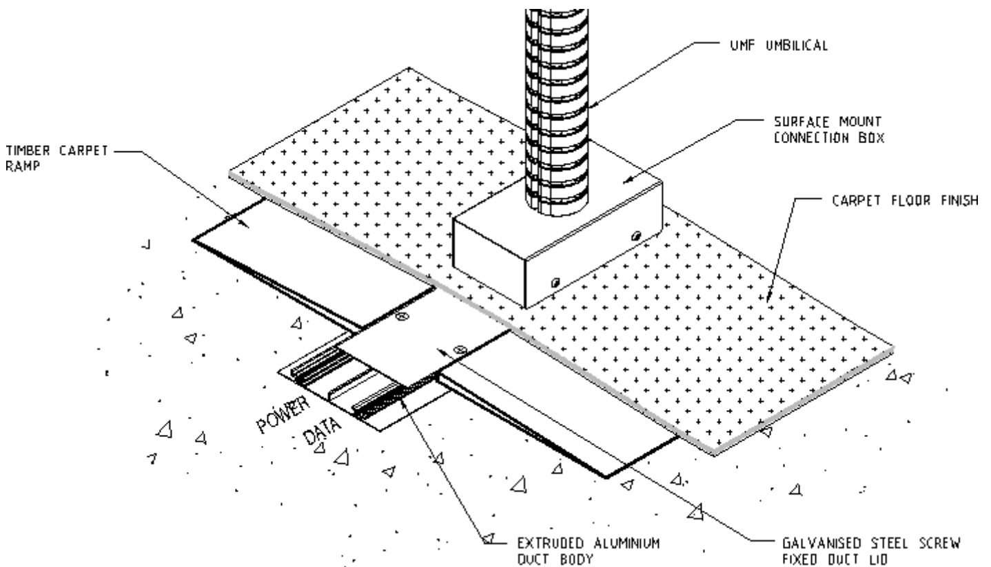
FFD10012DCR Adaptor box with Umbilical
