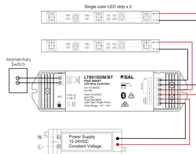
Wiring Diagram
