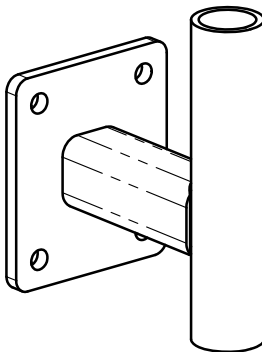
MB3-40-P-HG BRACKET
