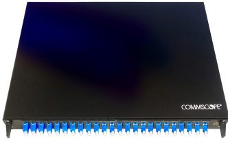
FMS Fiber Optic Termination/Splice Panel, 1U, 19 in, 48 LC/UPC, singlemode, OS2, black
