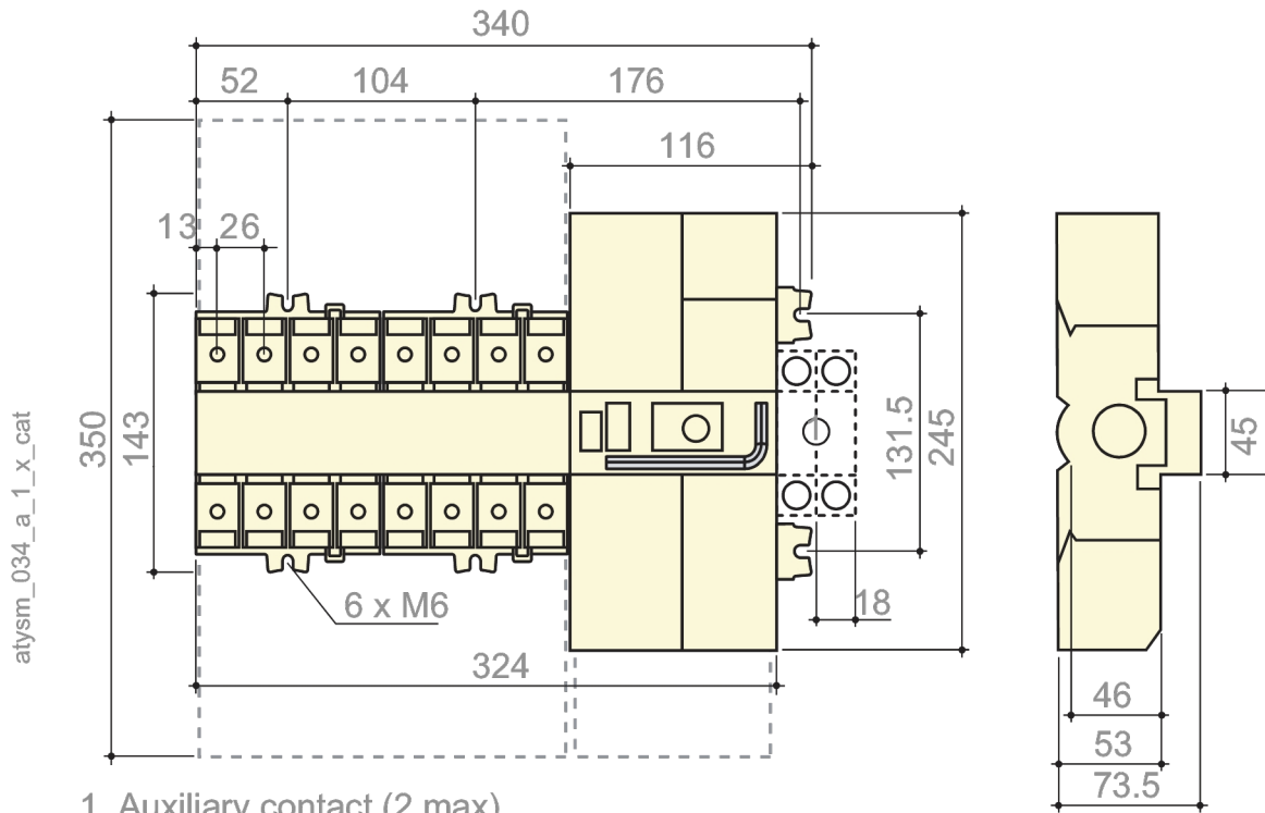
Dimension Diagram
