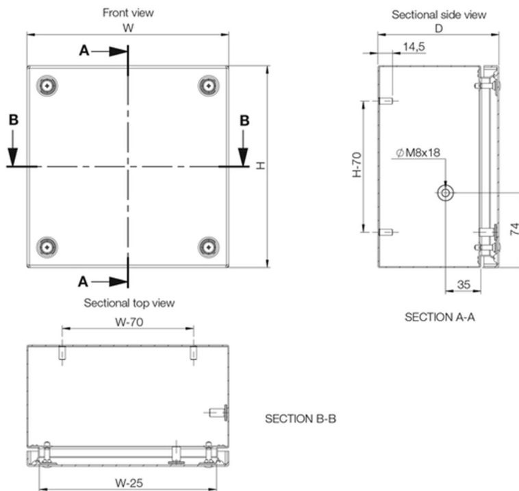
Dimension Diagram
