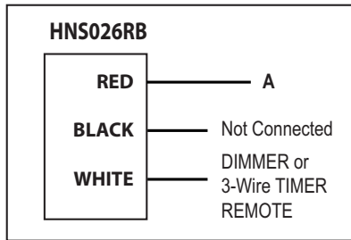
Figure 3: Button Only Operation (NO LED Indicator)
