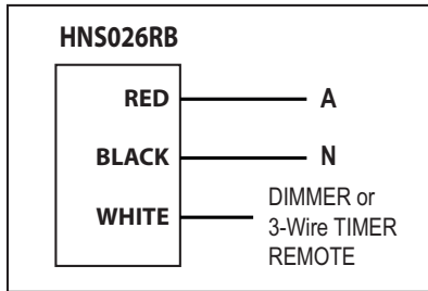
Figure 1: LED Indicator always ON
