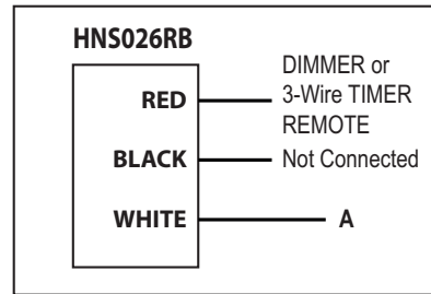
Figure 4: Button Only Operation (NO LED Indicator)
