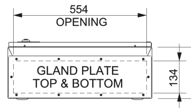
Plan view
