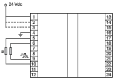
(1) Safety mat
