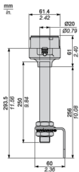
Dimensions for Metal Bracket
