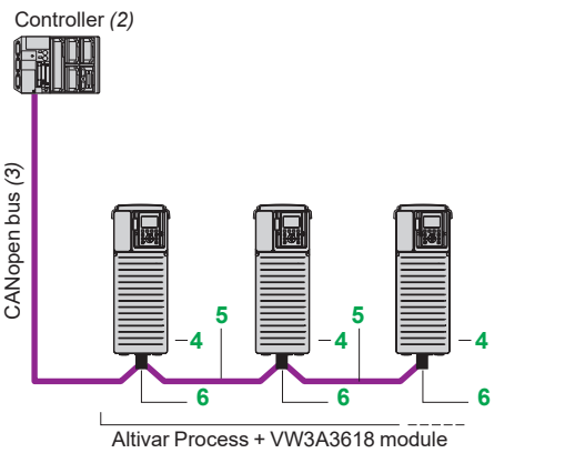
Example of connection to the CANopen bus via SUB-D connector
