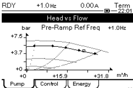
Altivar Process range
