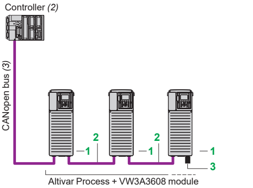
Optimized solution for daisy chain connection to the CANopen bus
