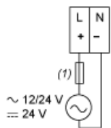
(1) Type T fuse (Controller: 1.25 A , Expansion: 1 A)
