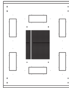
Top Panel 800w x 1000d
