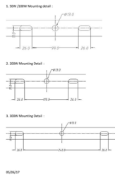
MAXI Master LED Flood GEN II Trunking Mounting Details.
