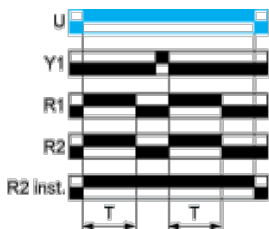
Function: 2 Outputs
