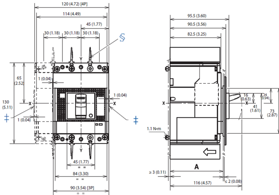
Dimension Diagram
