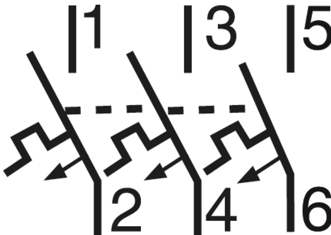
Connection / Wiring Diagram
