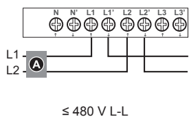
1PH2W LL
