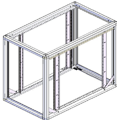
600w x 1200d Frame Assembly
