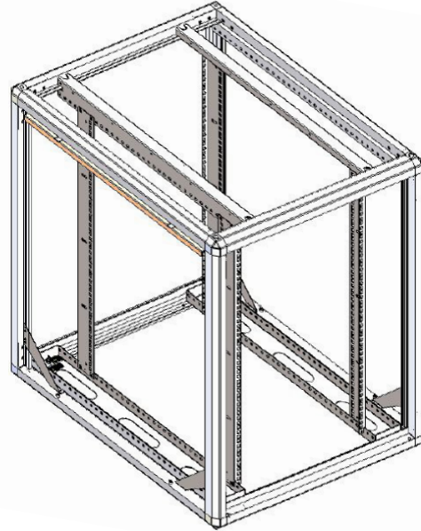
800w x 600d Frame Assembly
