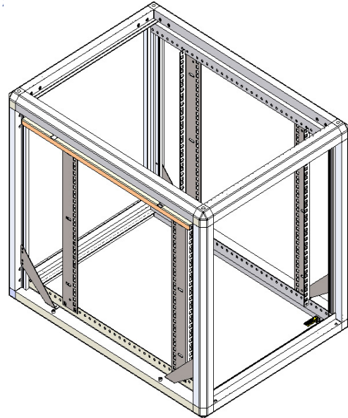
600w x 800d Frame Assembly
