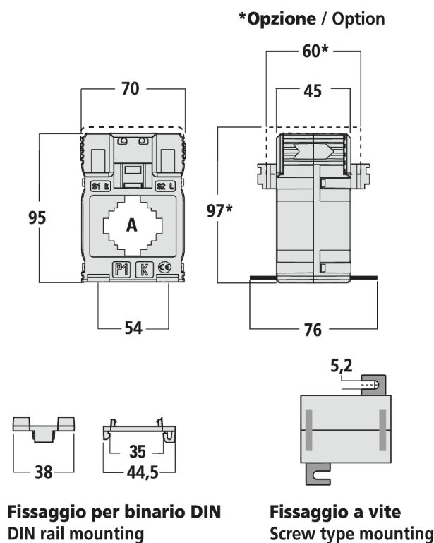
Dimension Diagram
